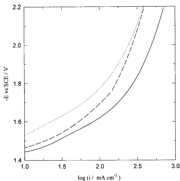
Fig. 2. Comparison of the current-potential relations for h.e.r. at different cathodes from 1\text{ M} KOH at 30\text{ }^\circ\text{C} . Key: ( \cdots ) Fe, ( --- ) Ni and ( --- ) Fe/PPy.
