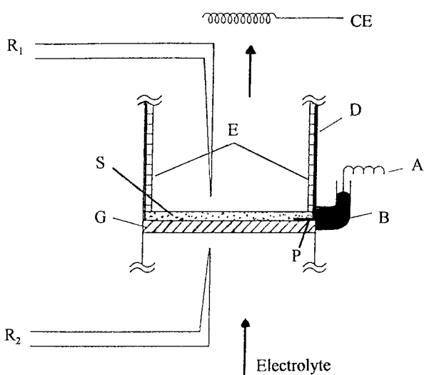
Fig. 1. Schematic diagram of the experimental arrangements for flow-through porous electrodes. Key: (A) connection to the current collector, (B) mercury connection; (D) cell wall, (E) rubber cylinder, (P) platinum current collector, (S) screen electrode (working electrode), (G) fritted glass disc, R1, R2; reference electrodes and (CE) counter electrode.
